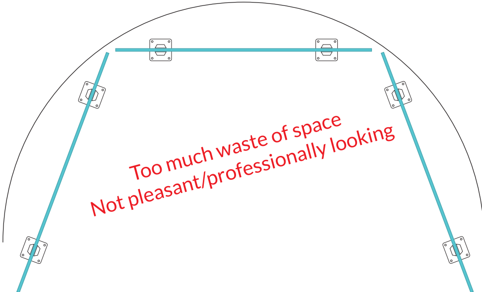
SHARP CURVE (or spiral) (Not suited for glass railings using straight glass panels)
